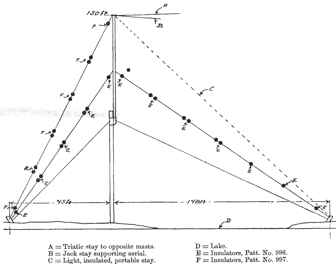
FIG. 2. Insulation of Horsea Masts.
