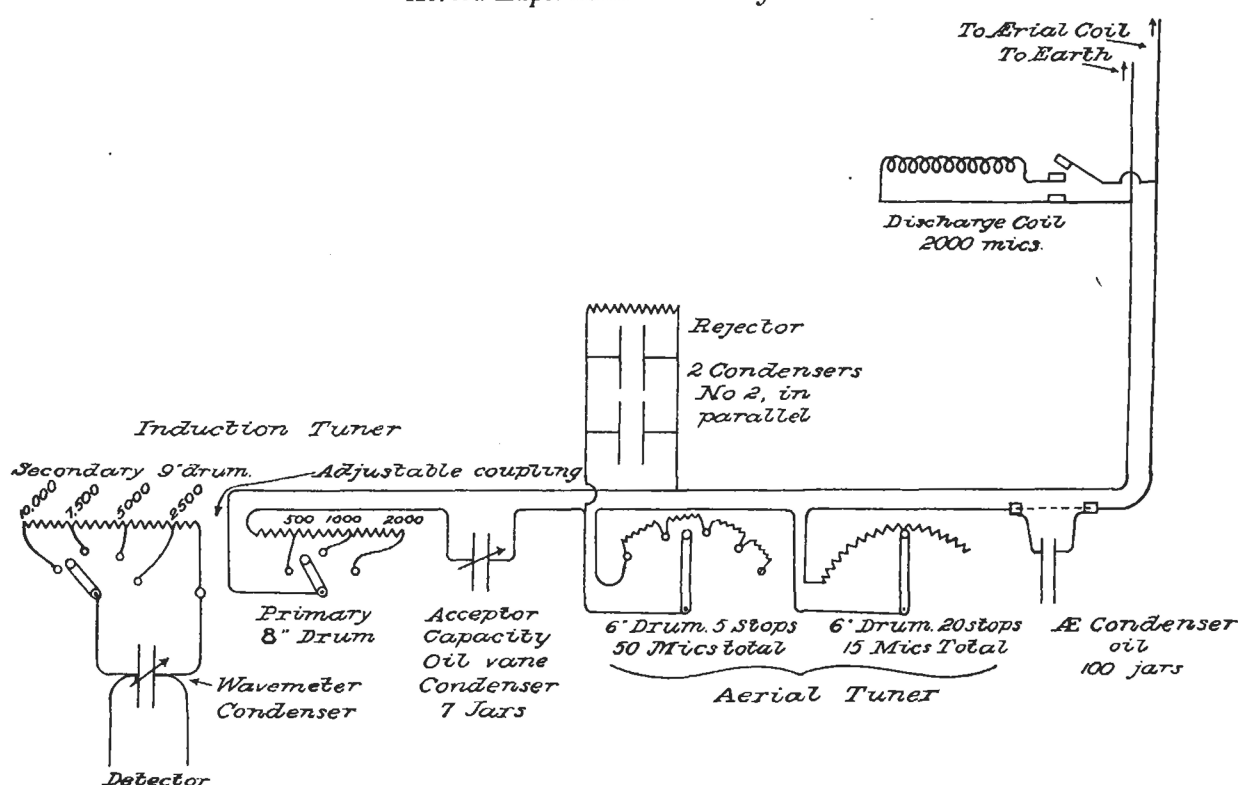
Horsea Experimental Receiving Gear.
