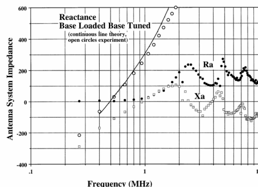
Fig. 4 Impedance vs. frequency for Marconi's temporary fan monopole December 1901 (experiment and simulation)
