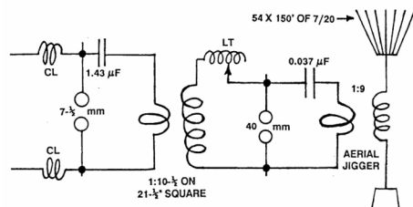
Fig. 3 Schematic showing component values for discharge circuit of the Poldhu transmitter in December 1901. Note the additional components C_L (extra coils), and L_T (a long adjustable tuning inductance of 40 turns using 40 feet of wire). From Fleming's Notebook (after Thackeray [3]).
