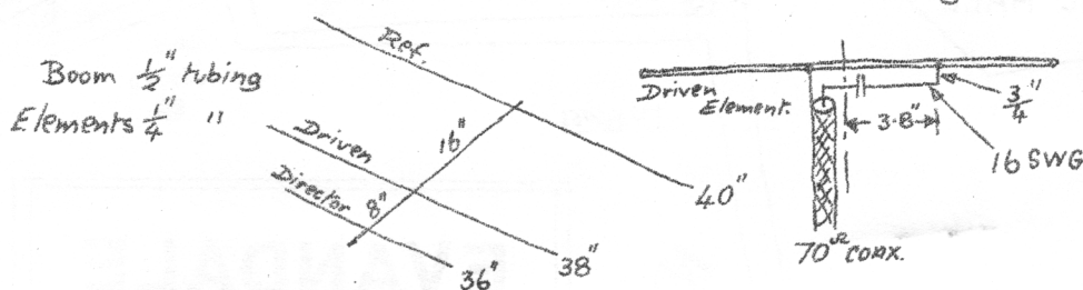
144 MHz 3 Element Yagi Suitable for VHF Fox Hunting
