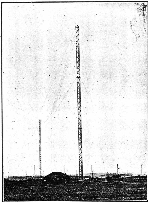
3LO's aerial itself—a magnificent affair 200 feet high—is directly responsible for the creation of the ether waves.
