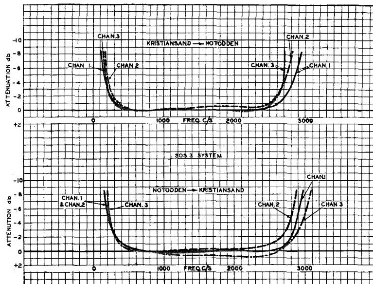
Fig. 14—Overall Quality—Notodden-Kristiansand.
