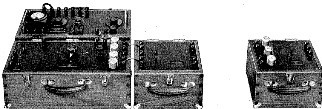
Fig. 3—74101-A Crosstalk Set, Amplifier, PH-S Unit and Terminating Unit.
