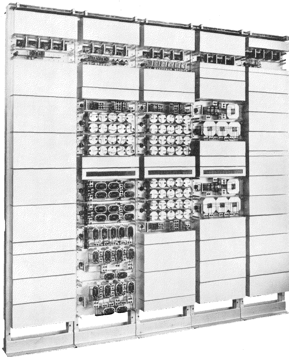
Fig. 5—SOT.3 Terminal. Rear View with Covers Removed.
