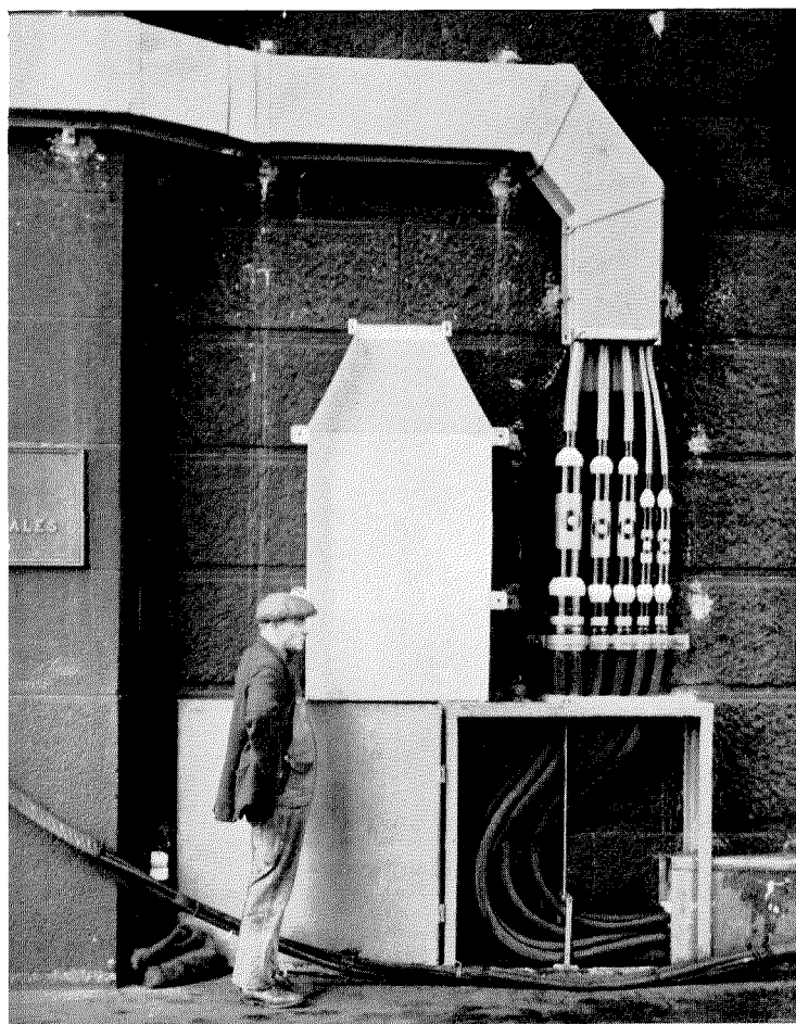
Fig. 7—Forth Bridge—Joints and Slack Box at South Pier.
