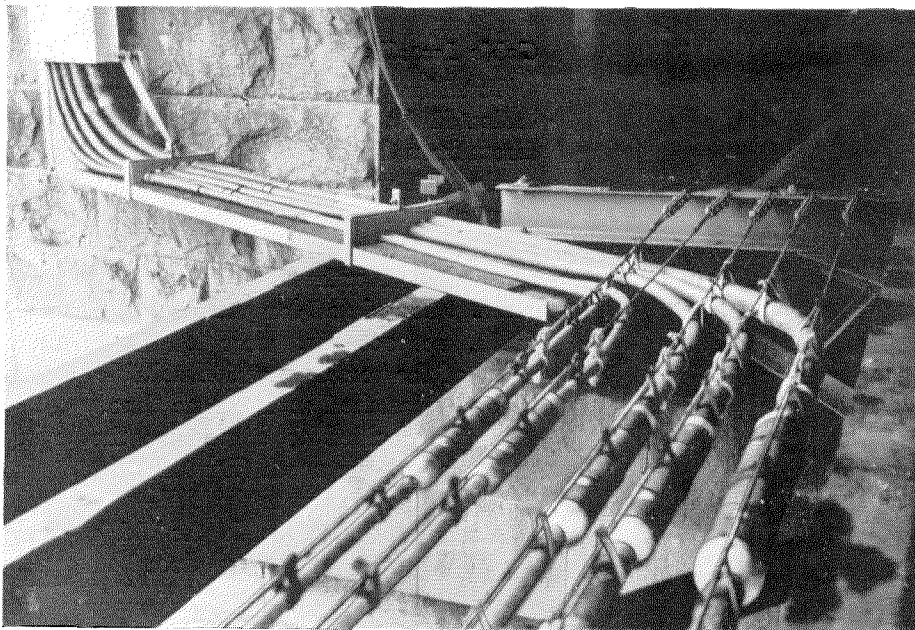
Fig. 3—Forth Bridge — End of horizontal aerial run on G.I. strand on south viaduct and commencement of rise on south pier.
