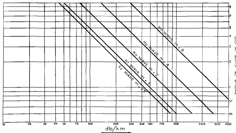
Plate I—Attenuation due to dielectric loss (assuming \tan \theta = 2.10^{-4} ).
